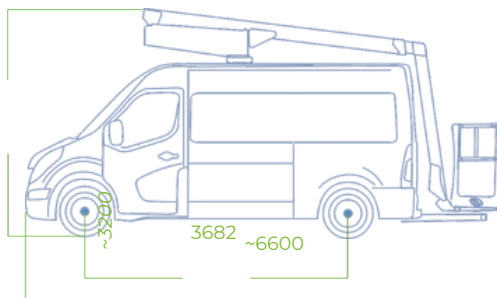
Renault Master
