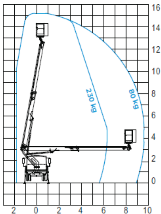
SURFACE MAXIMALE
